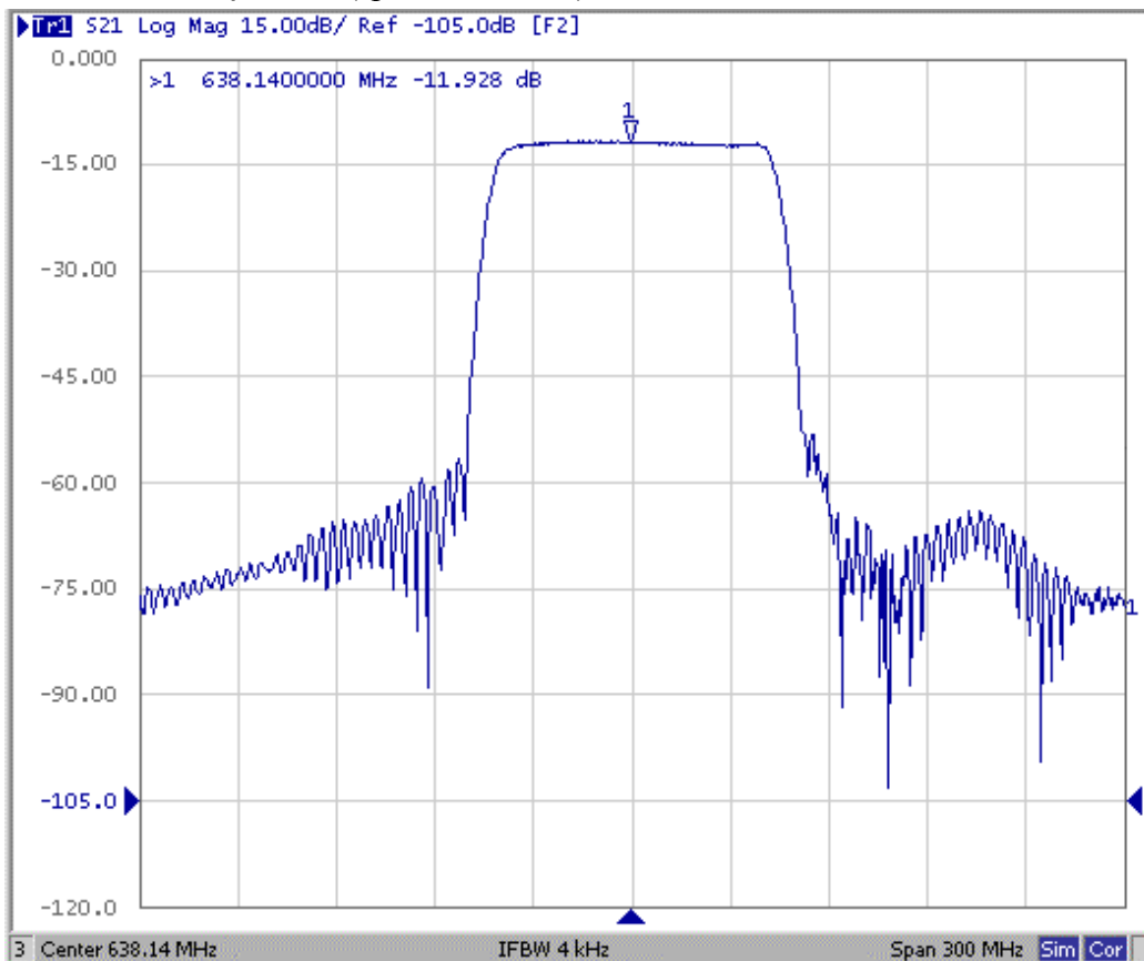
Fig1. Horizontal: 30MHz/Div Vertical: 15dB/Div
